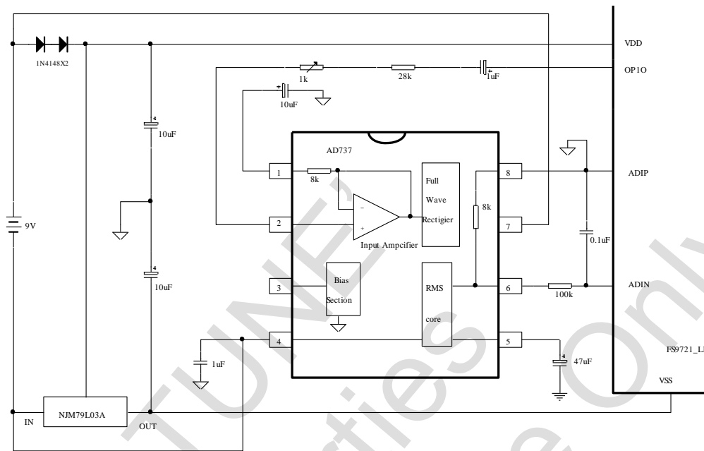
Diagram 23 True Valid Value Rectification Circuitry
