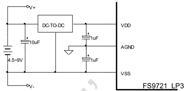
Diagram 11 4.5V~9V Power Supply
