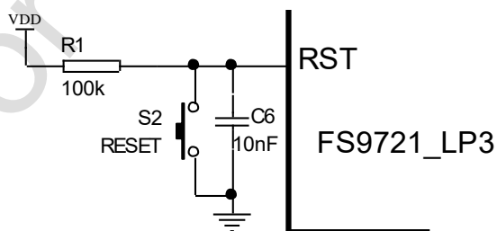
Diagram 16 Reset Circuit
