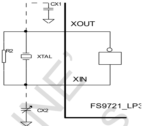
Diagram 17 Quartz Oscillation Circuit
