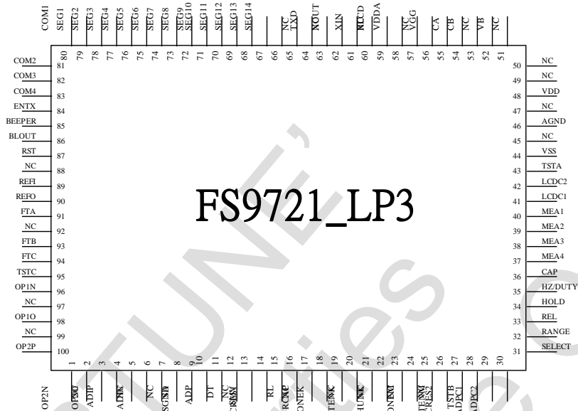
Diagram 2 100PIN Package
