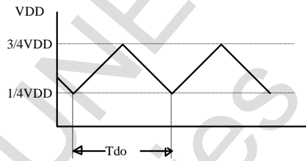
Diagram 31 Capacitance Measurement
