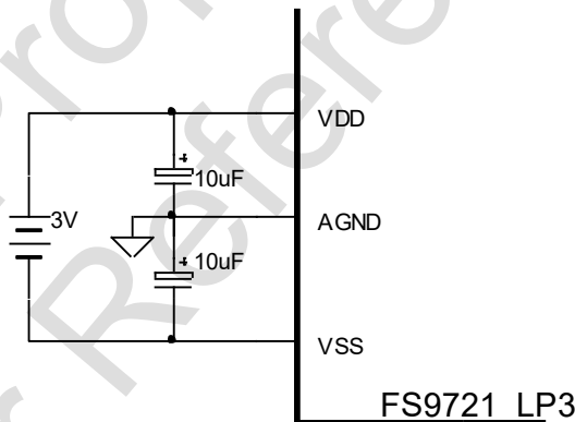
Diagram 10 3V Power Supply
