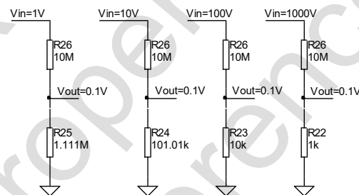
Diagram 25 Voltage Division Circuitry
