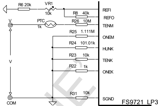
Diagram 24 Voltage Measurement
